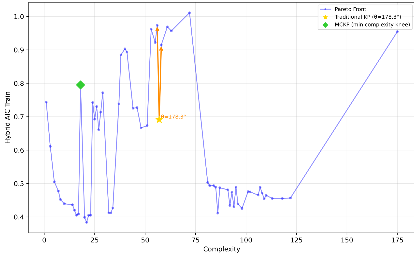
192_vineyard - Run 21 - MVP - Hybrid AIC Train \lambda_1=0.00, \lambda_2=0.30, \lambda_3=1.00 | Difficulty: 0.23 | Method: mckp
