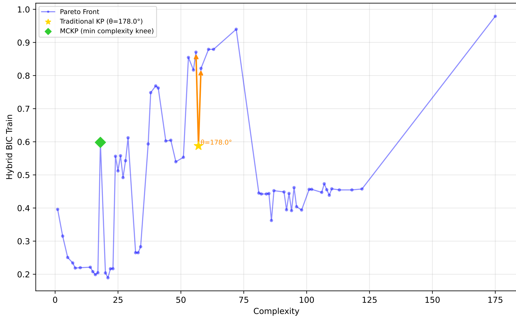
192_vineyard - Run 21 - MVP - Hybrid BIC Train \lambda_1=0.00, \lambda_2=0.30, \lambda_3=1.00 | Difficulty: 0.23 | Method: mckp
