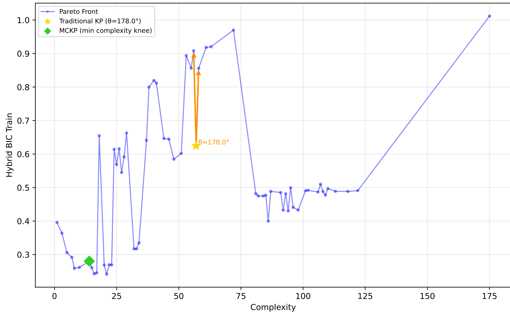
192_vineyard - Run 21 - MVP - Hybrid BIC Train \lambda_1=0.40, \lambda_2=0.00, \lambda_3=1.00 | Difficulty: 0.23 | Method: mckp
