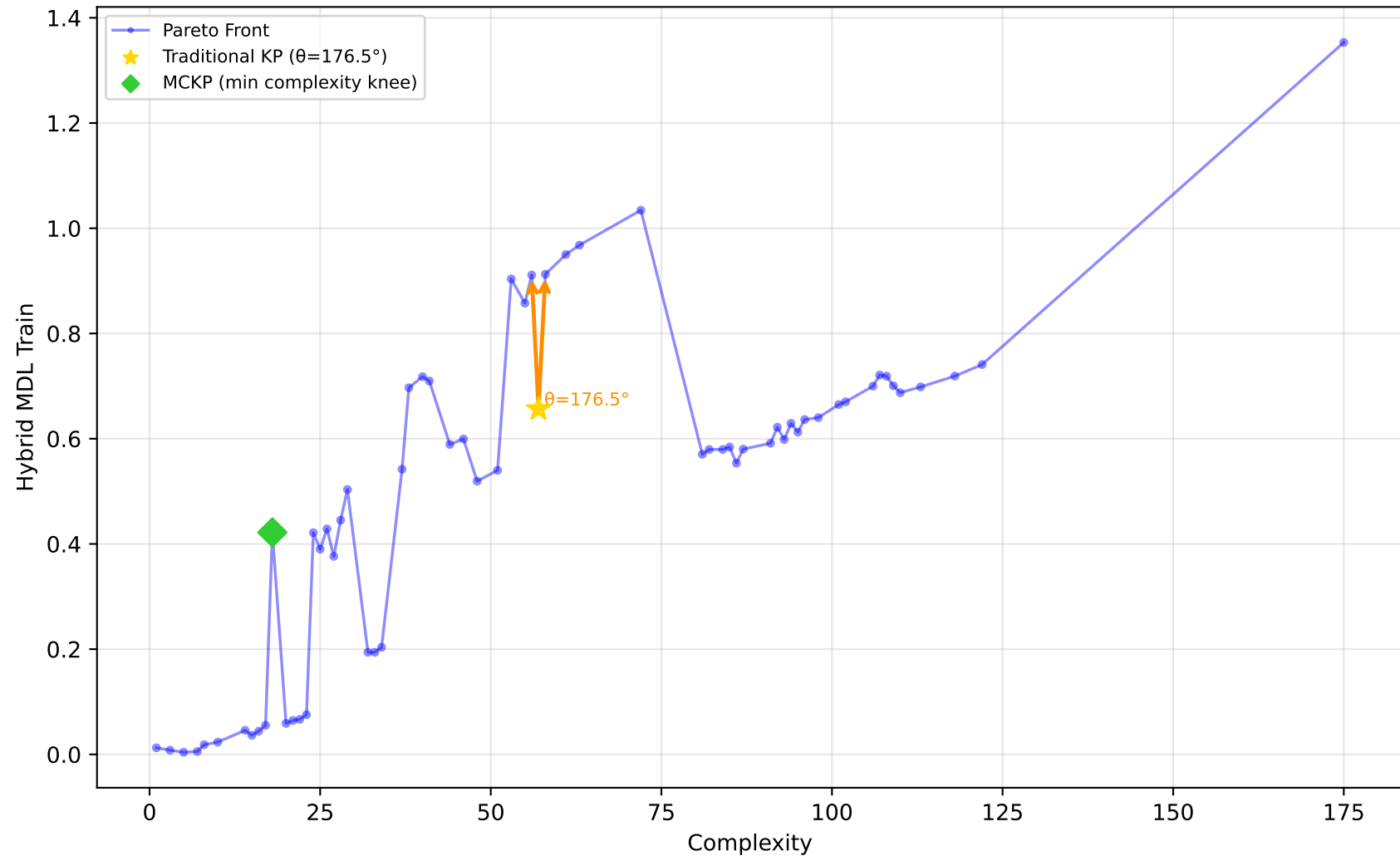
192_vineyard - Run 21 - MVP - Hybrid MDL Train \lambda_1=0.00, \bar{\lambda}_2=0.30, \lambda_3=1.00 | Difficulty: 0.23 | Method: mckp
