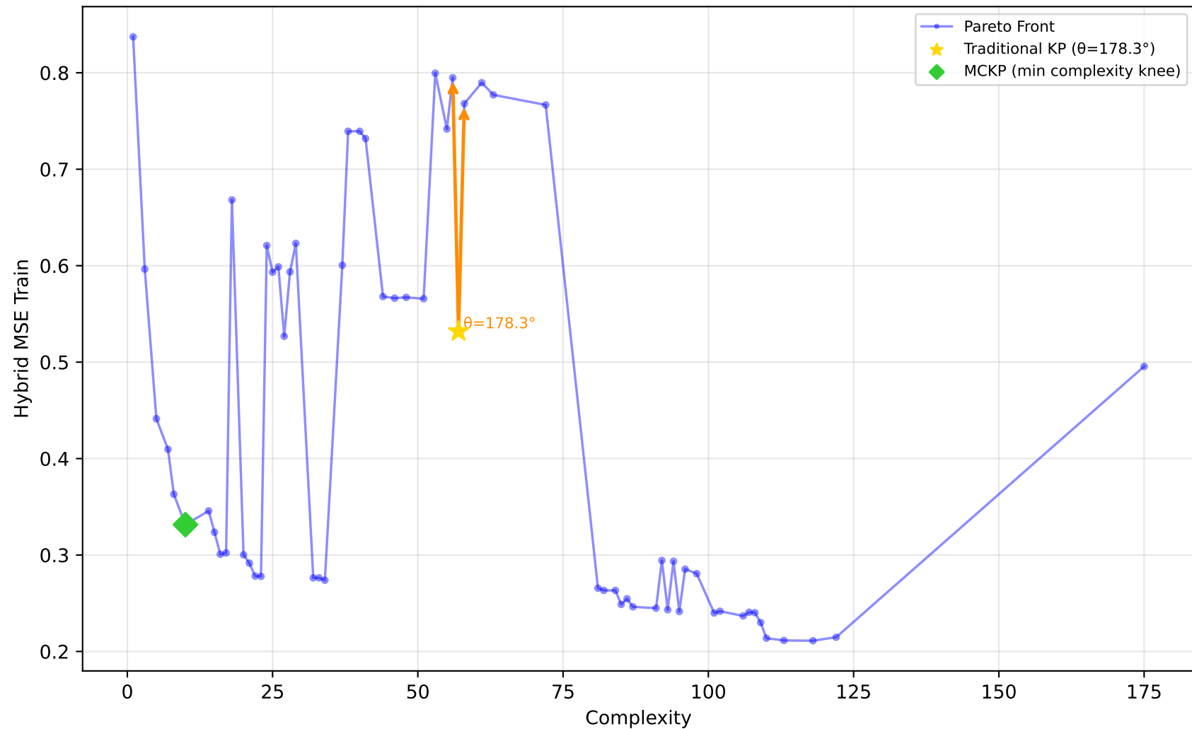
192_vineyard - Run 21 - MVP - Hybrid MSE Train \lambda_1=0.40, \bar{\lambda}_2=0.00, \lambda_3=1.00 | Difficulty: 0.23 | Method: mckp
