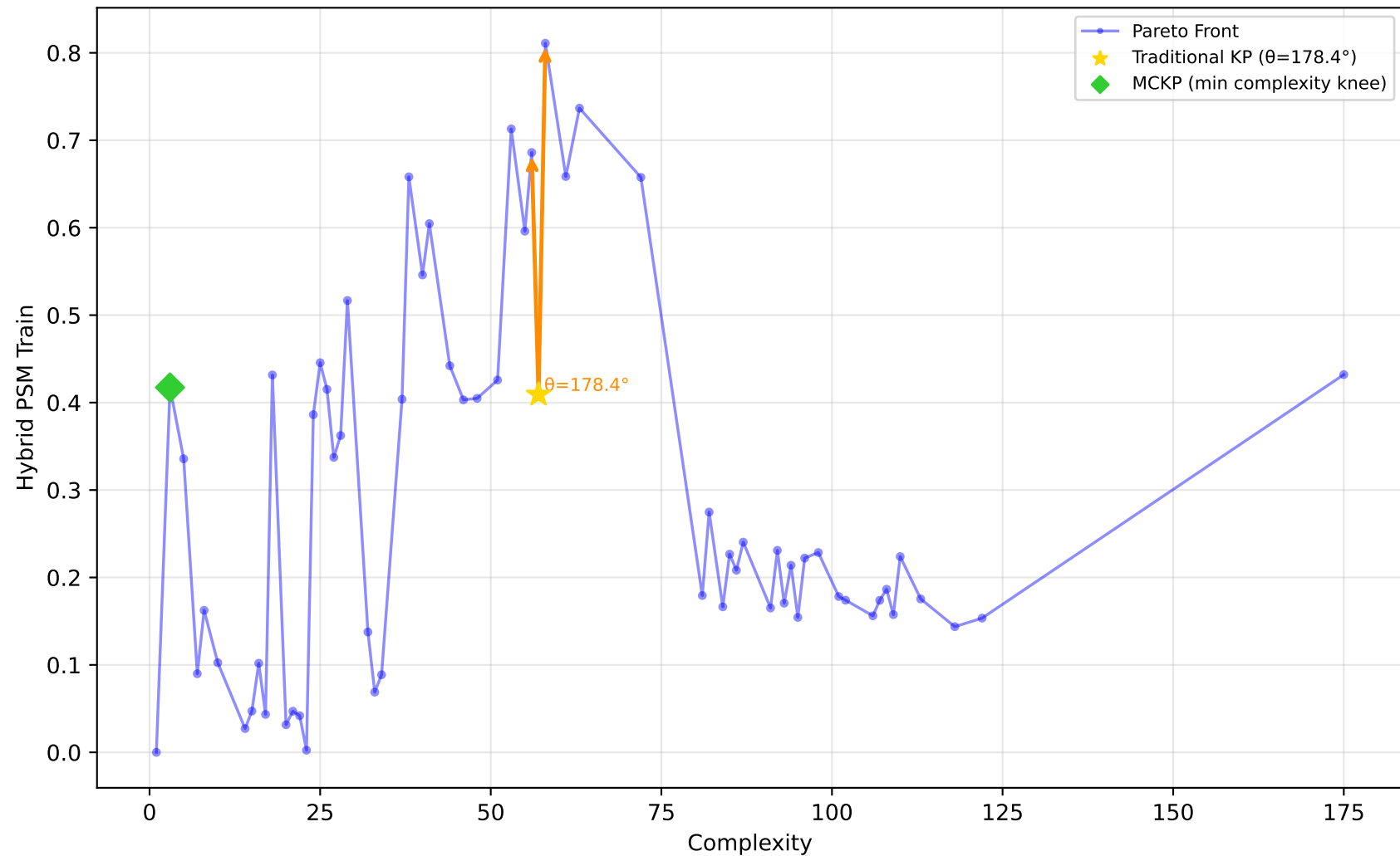
192_vineyard - Run 21 - MVP - Hybrid PSM Train \lambda_1=0.00, \lambda_2=0.30, \lambda_3=1.00 | Difficulty: 0.23 | Method: mckp
