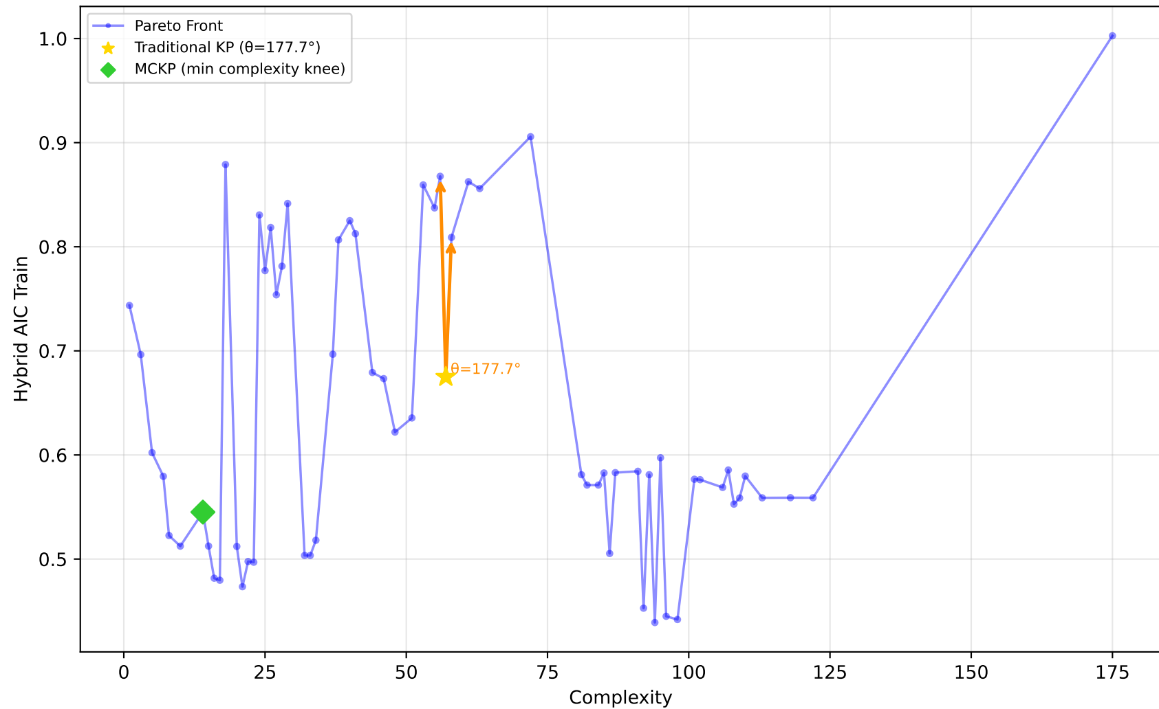
192_vineyard - Run 21 - SVP - Hybrid AIC Train \lambda_1=0.70, \lambda_2=0.70, \lambda_3=0.90 | Difficulty: 0.23 | Method: mckp
