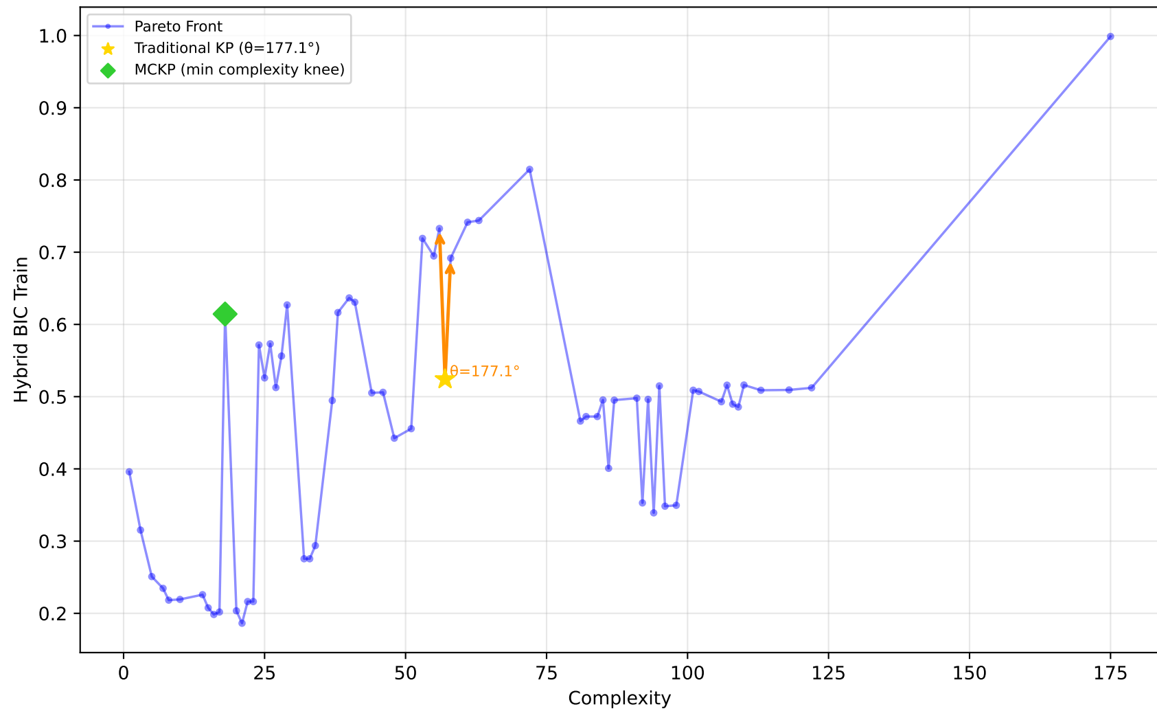
192_vineyard - Run 21 - SVP - Hybrid BIC Train \lambda_1=0.00, \lambda_2=1.00, \lambda_3=1.00 | Difficulty: 0.23 | Method: mckp
