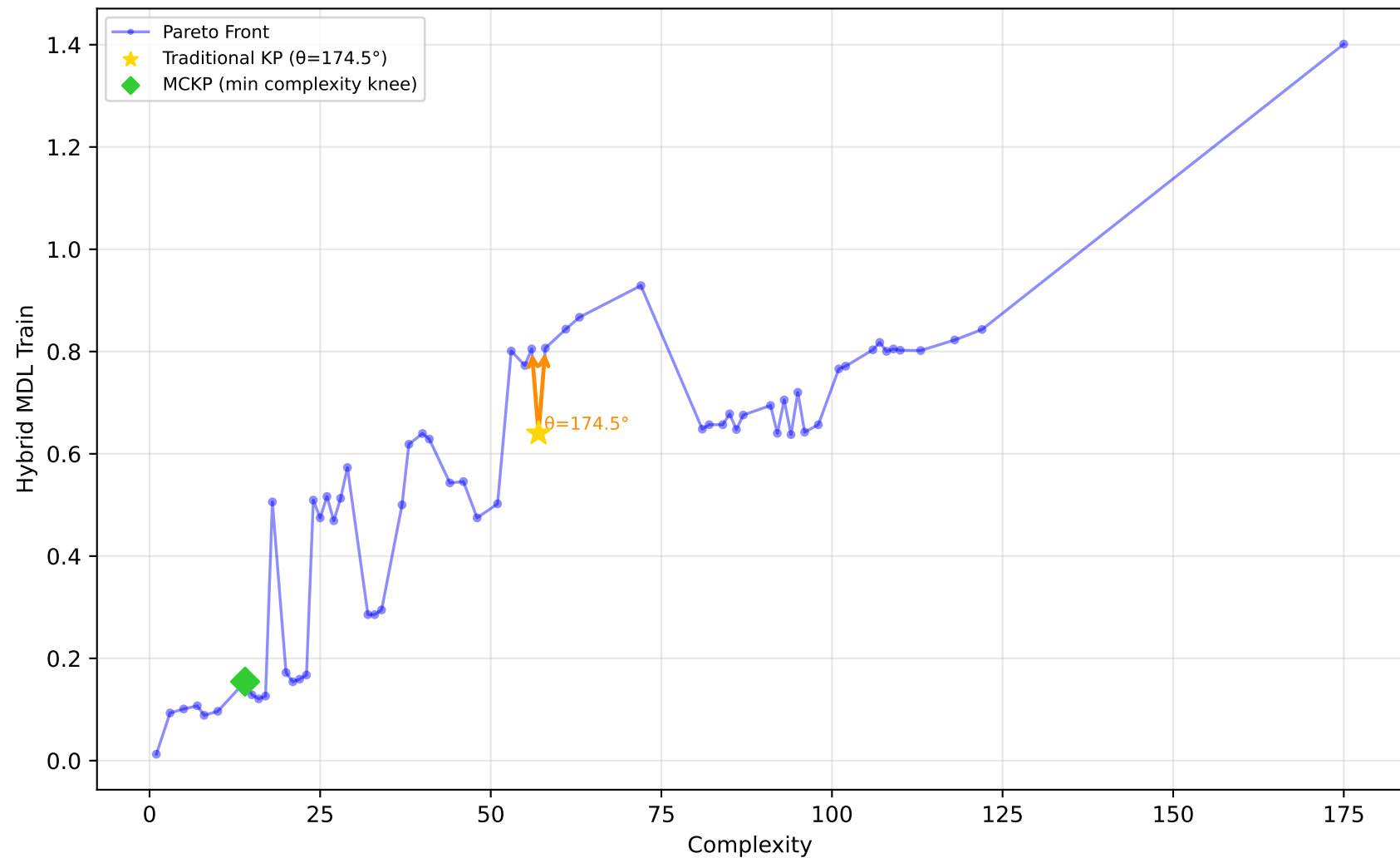
192_vineyard - Run 21 - SVP - Hybrid MDL Train \lambda_1=0.70, \bar{\lambda}_2=0.70, \lambda_3=0.90 | Difficulty: 0.23 | Method: mckp
