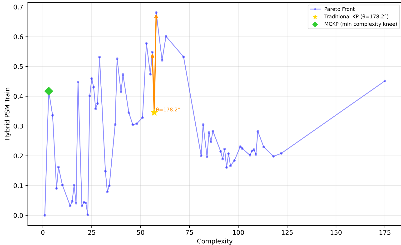
192_vineyard - Run 21 - SVP - Hybrid PSM Train \lambda_1=0.00, \lambda_2=1.00, \lambda_3=1.00 | Difficulty: 0.23 | Method: mckp
