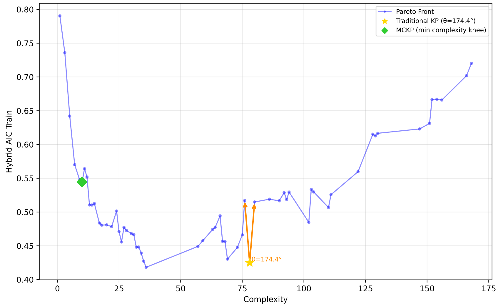
192_vineyard - Run 22 - MVP - Hybrid AIC Train \lambda_1=0.40, \bar{\lambda}_2=0.00, \lambda_3=1.00 | Difficulty: 1.00 | Method: hmr
