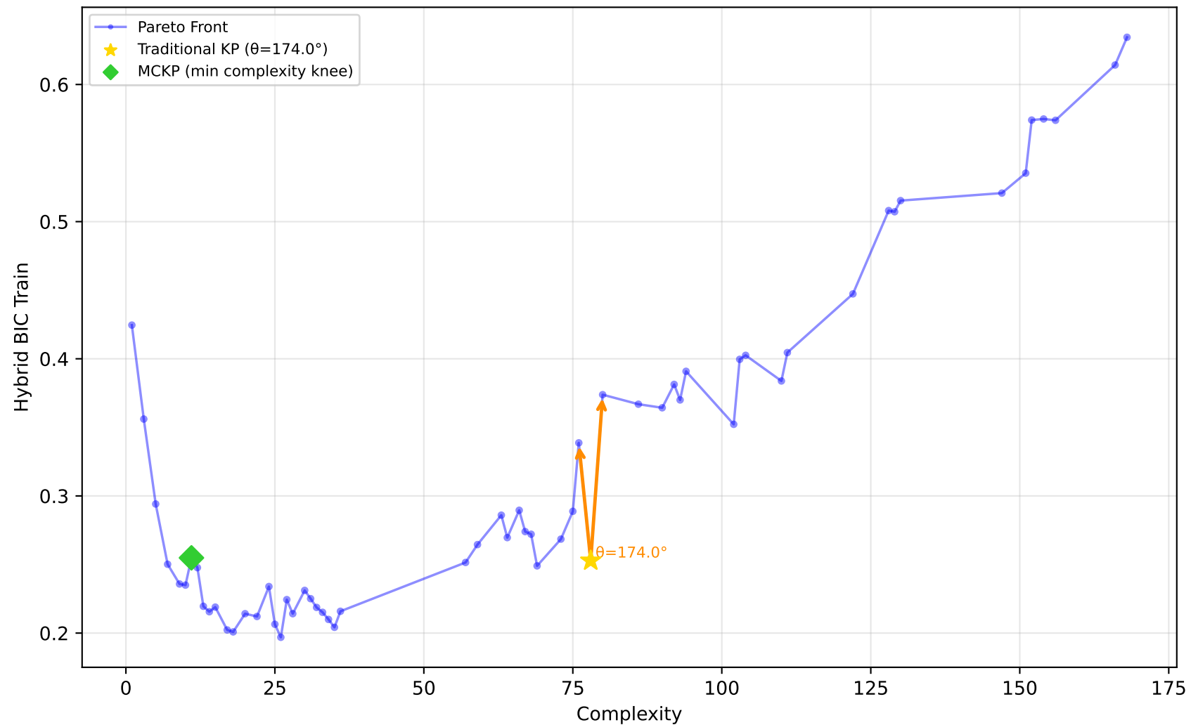
192_vineyard - Run 22 - MVP - Hybrid BIC Train \lambda_1=0.00, \bar{\lambda}_2=0.30, \lambda_3=1.00 | Difficulty: 1.00 | Method: hmr
