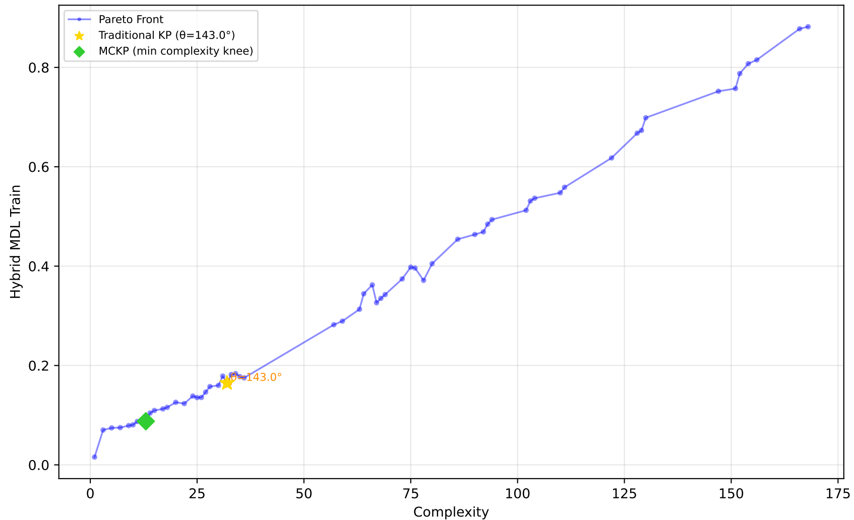
192_vineyard - Run 22 - MVP - Hybrid MDL Train \lambda_1=0.40, \bar{\lambda}_2=0.00, \lambda_3=1.00 | Difficulty: 1.00 | Method: hmr
