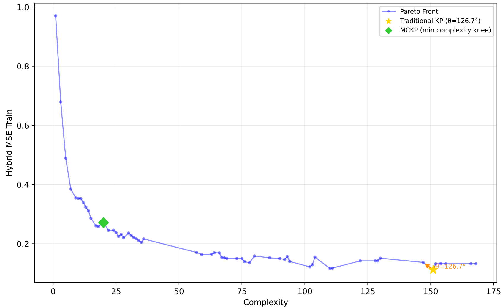
192_vineyard - Run 22 - MVP - Hybrid MSE Train \lambda_1=0.00, \bar{\lambda}_2=0.30, \lambda_3=1.00 | Difficulty: 1.00 | Method: hmr
