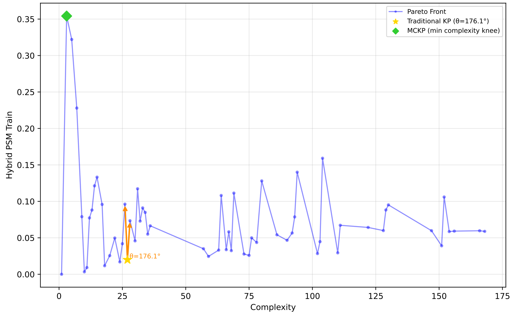
192_vineyard - Run 22 - MVP - Hybrid PSM Train \lambda_1=0.00, \bar{\lambda}_2=0.30, \lambda_3=1.00 | Difficulty: 1.00 | Method: hmr
