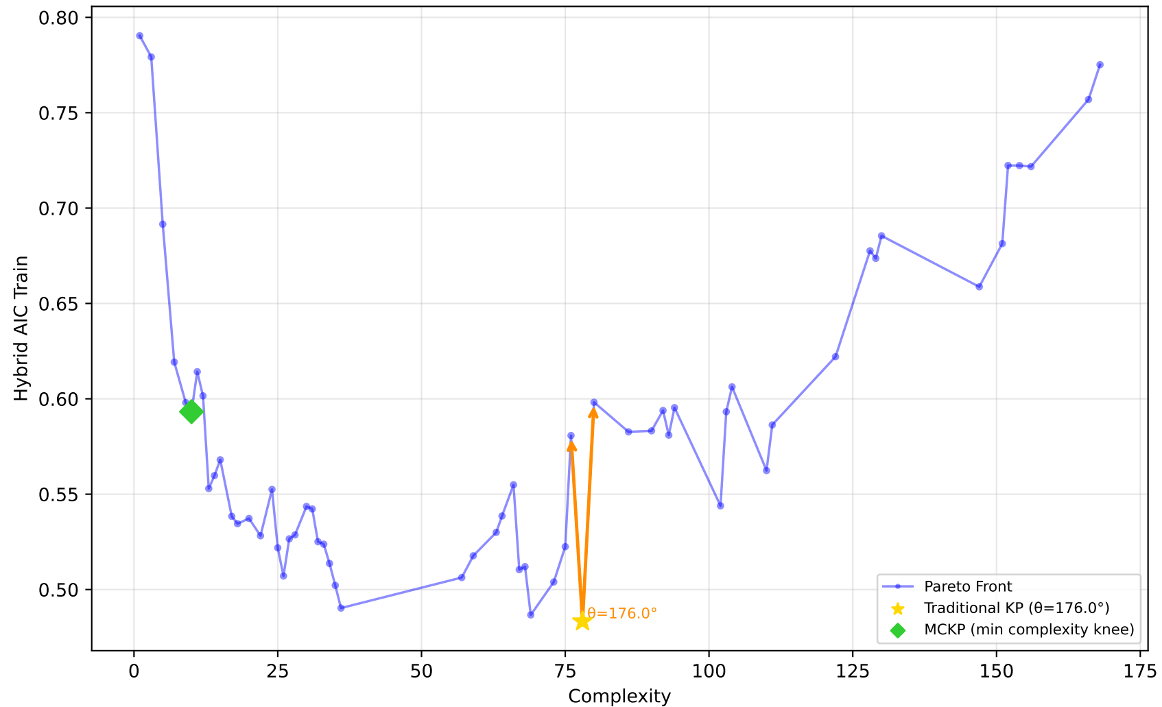
192_vineyard - Run 22 - SVP - Hybrid AIC Train \lambda_1=0.70, \bar{\lambda}_2=0.70, \lambda_3=0.90 | Difficulty: 1.00 | Method: hmr
