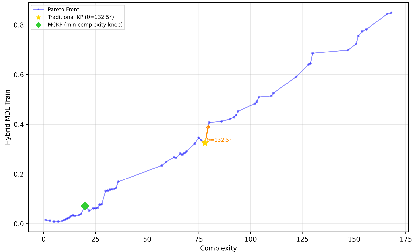
192_vineyard - Run 22 - SVP - Hybrid MDL Train \lambda_1=0.00, \bar{\lambda}_2=1.00, \lambda_3=1.00 | Difficulty: 1.00 | Method: hmr
