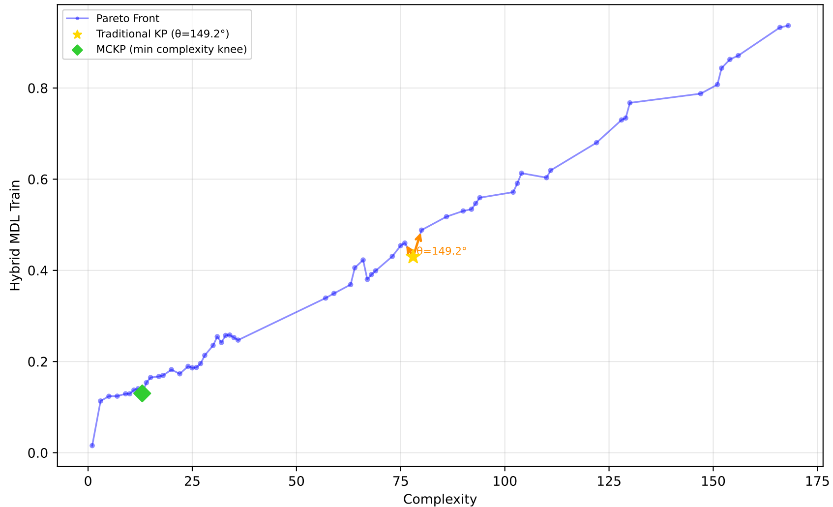
192_vineyard - Run 22 - SVP - Hybrid MDL Train \lambda_1=0.70, \bar{\lambda}_2=0.70, \lambda_3=0.90 | Difficulty: 1.00 | Method: hmr
