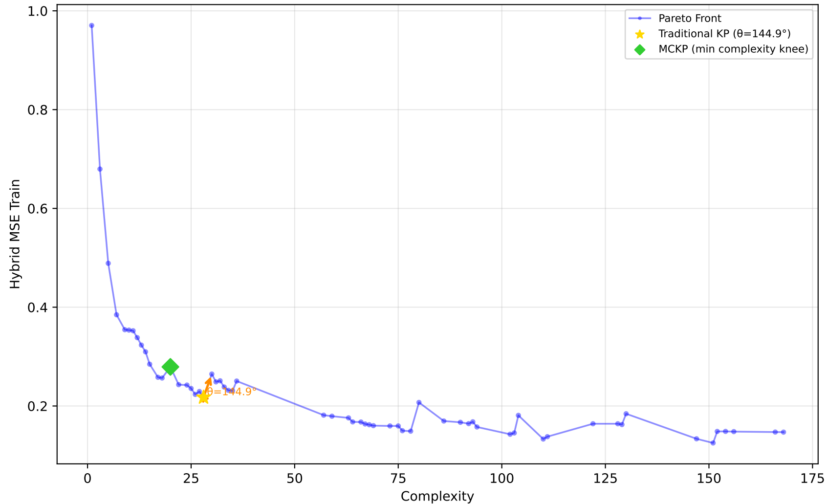
192_vineyard - Run 22 - SVP - Hybrid MSE Train \lambda_1=0.00, \bar{\lambda}_2=1.00, \lambda_3=1.00 | Difficulty: 1.00 | Method: hmr
