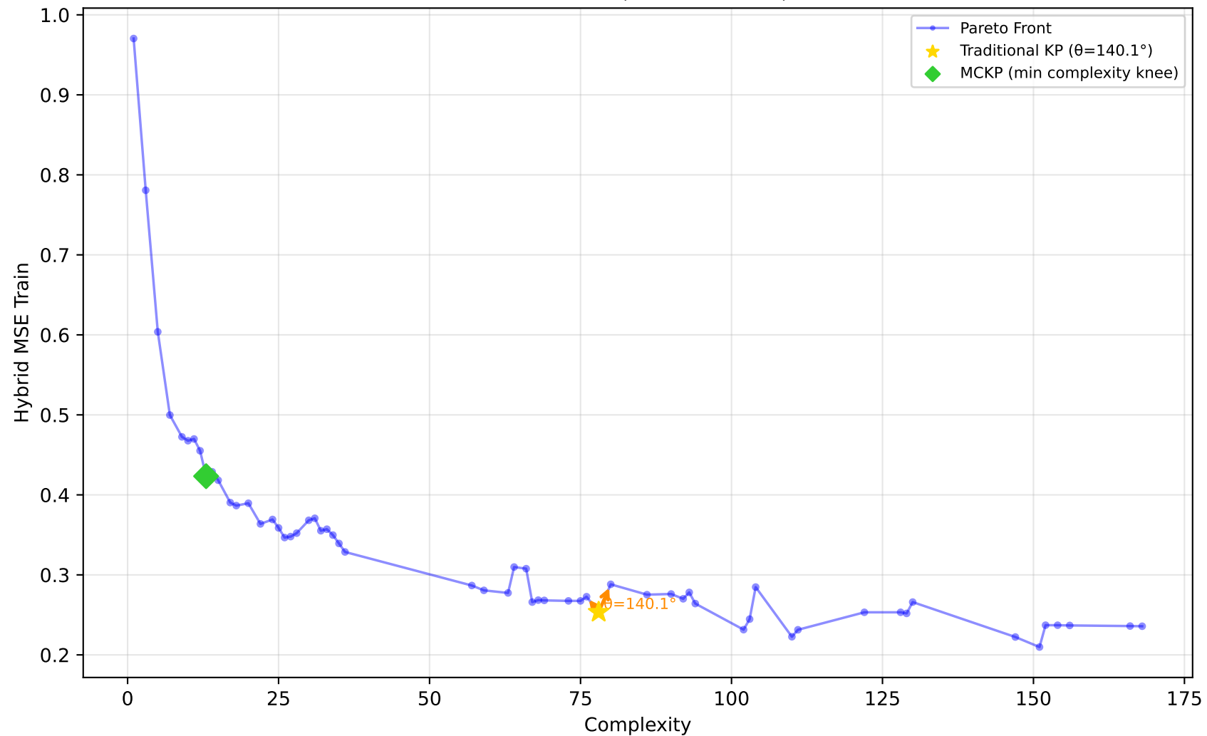
192_vineyard - Run 22 - SVP - Hybrid MSE Train \lambda_1=0.70, \bar{\lambda}_2=0.70, \lambda_3=0.90 | Difficulty: 1.00 | Method: hmr
