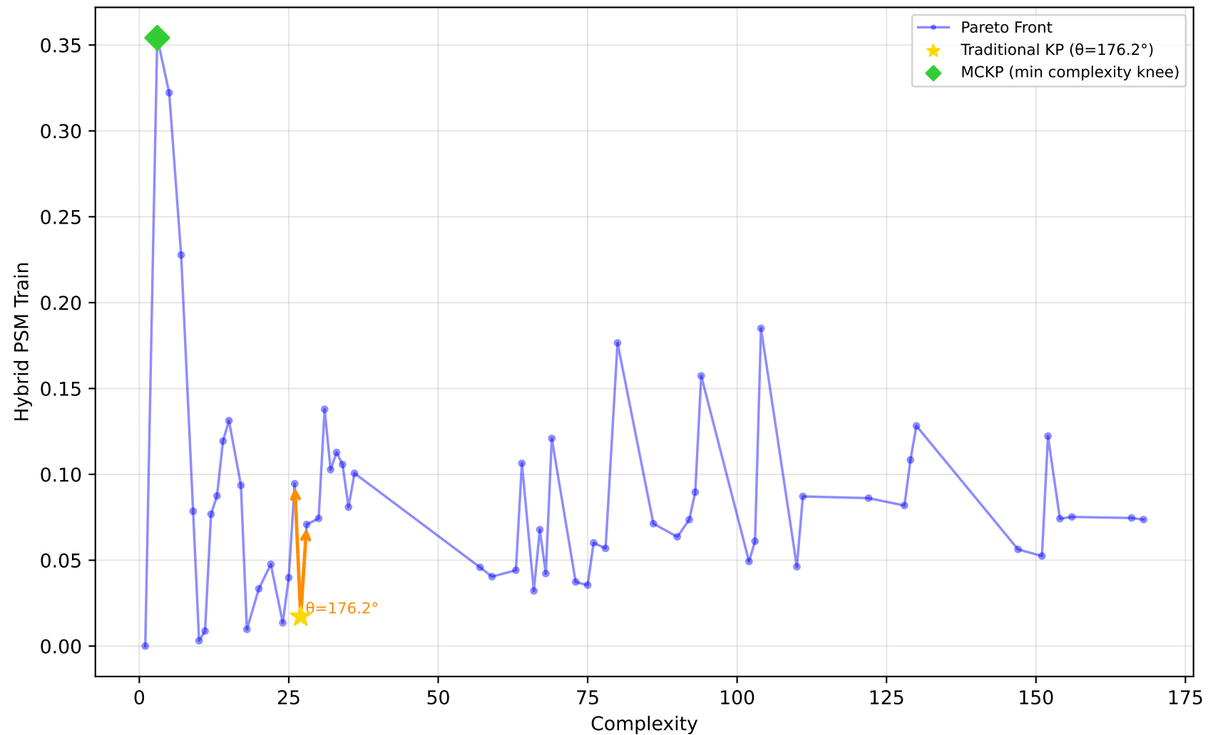
192_vineyard - Run 22 - SVP - Hybrid PSM Train \lambda_1=0.00, \bar{\lambda}_2=1.00, \lambda_3=1.00 | Difficulty: 1.00 | Method: hmr
