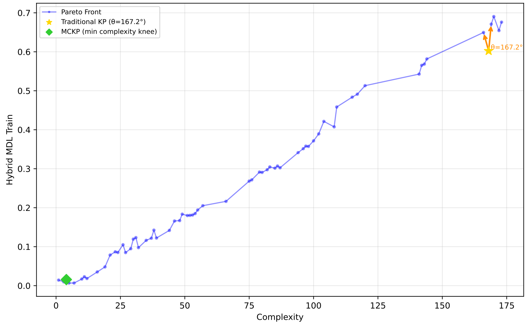
192_vineyard - Run 23 - MVP - Hybrid MDL Train \lambda_1=0.00, \bar{\lambda}_2=0.30, \lambda_3=1.00 | Difficulty: 0.67 | Method: hmr
