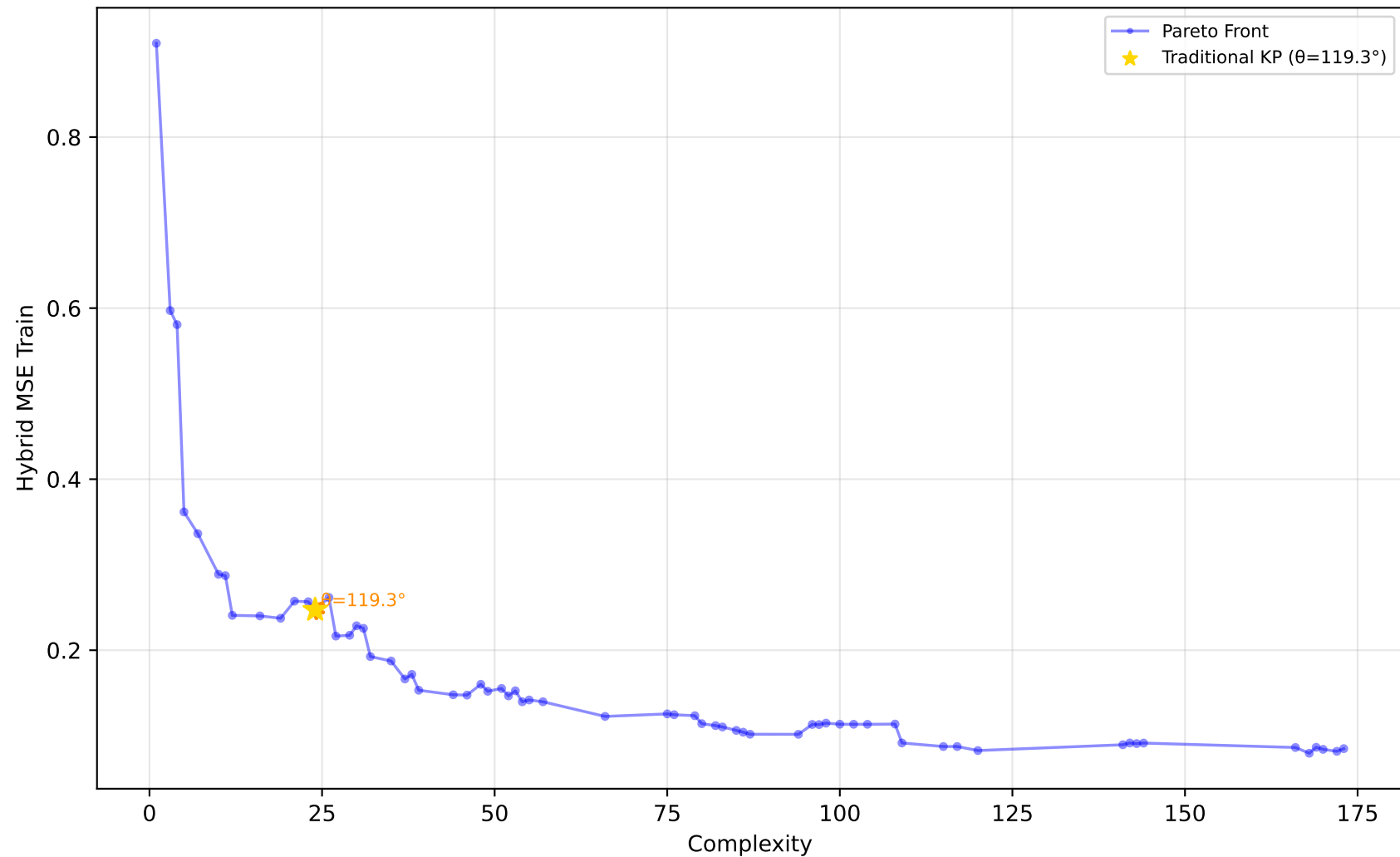
192_vineyard - Run 23 - MVP - Hybrid MSE Train \lambda_1=0.00, \lambda_2=0.30, \lambda_3=1.00 | Difficulty: 0.67 | Method: hmr
