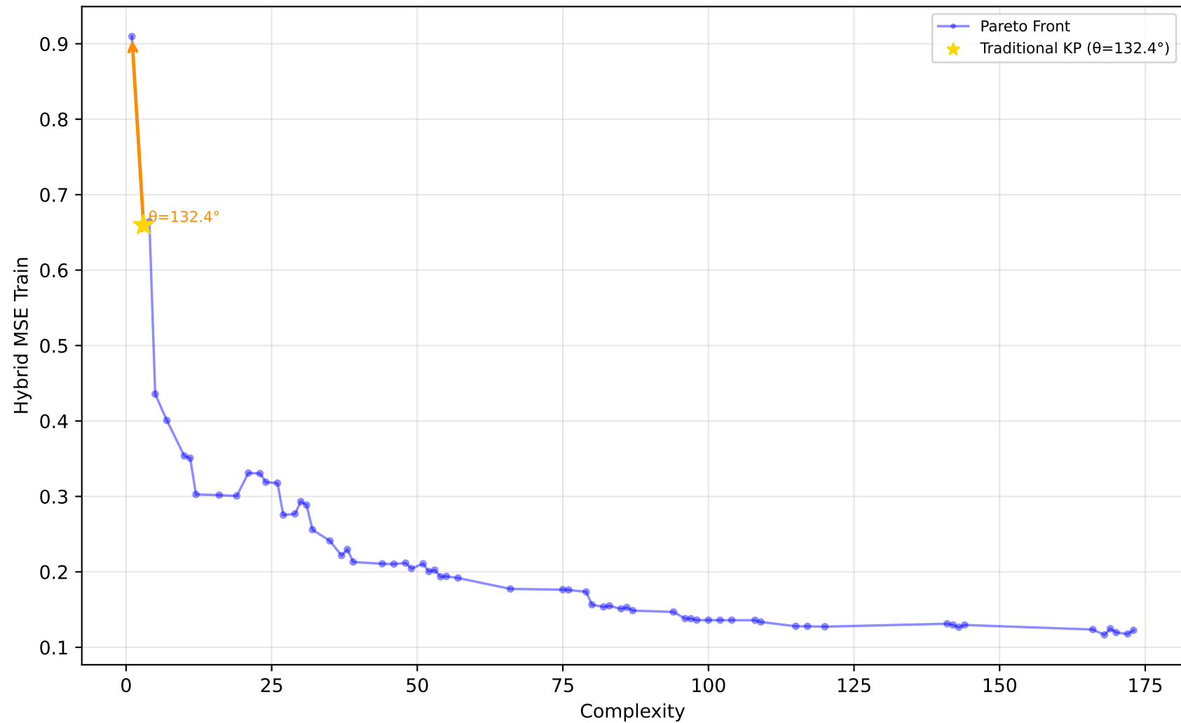
192_vineyard - Run 23 - MVP - Hybrid MSE Train \lambda_1=0.40, \lambda_2=0.00, \lambda_3=1.00 | Difficulty: 0.67 | Method: hmr
