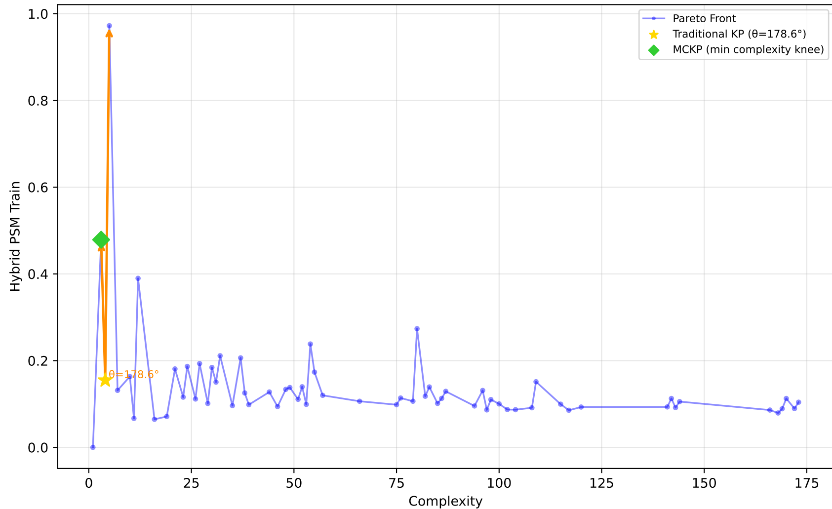
192_vineyard - Run 23 - MVP - Hybrid PSM Train \lambda_1=0.40, \lambda_2=0.00, \lambda_3=1.00 | Difficulty: 0.67 | Method: hmr
