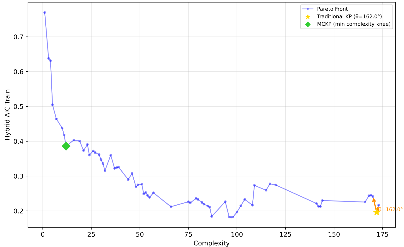
192_vineyard - Run 23 - SVP - Hybrid AIC Train \lambda_1=0.00, \bar{\lambda}_2=1.00, \lambda_3=1.00 | Difficulty: 0.67 | Method: hmr
