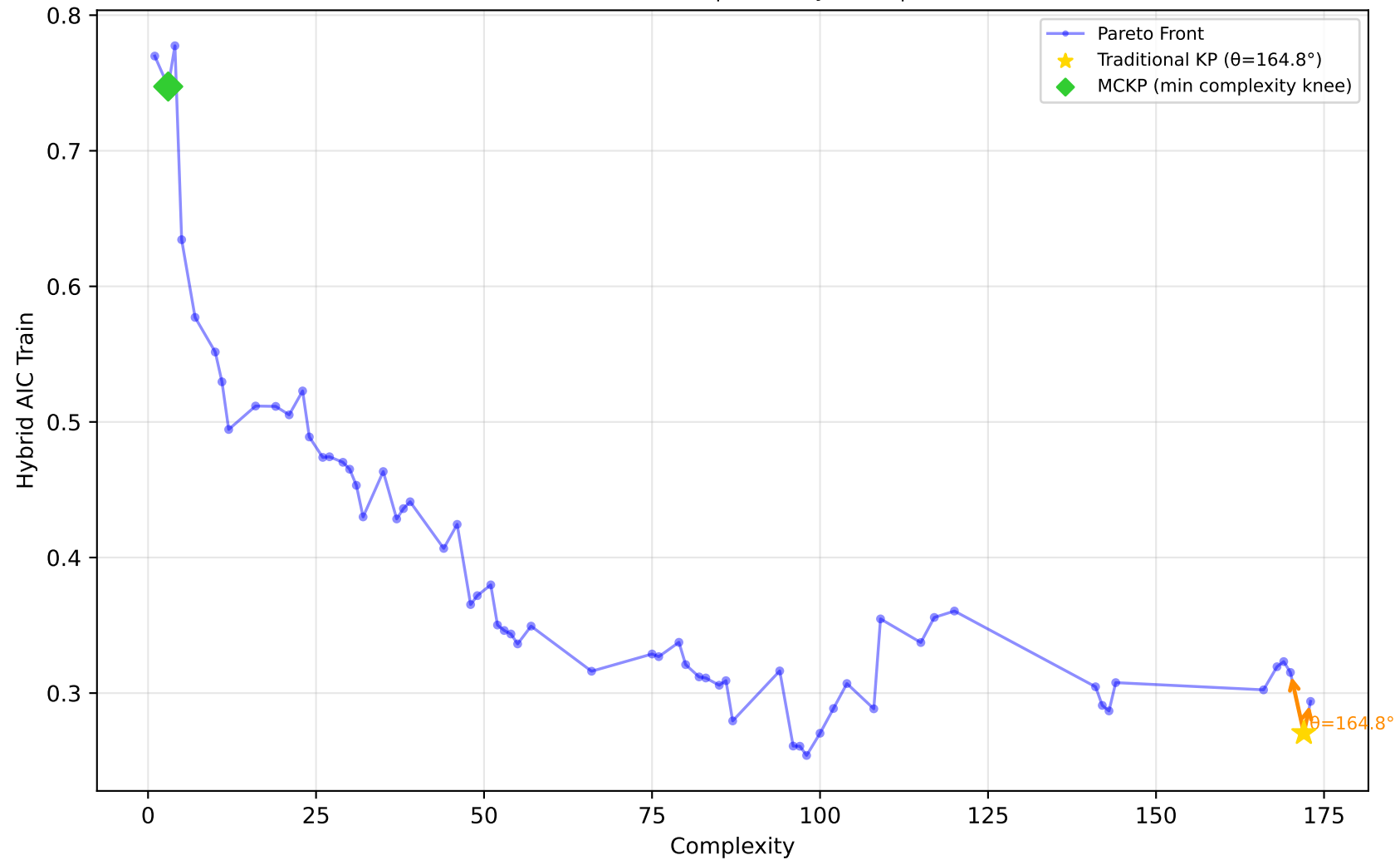
192_vineyard - Run 23 - SVP - Hybrid AIC Train \lambda_1=0.70 , \lambda_2=0.70 , \lambda_3=0.90 | Difficulty: 0.67 | Method: hmr
