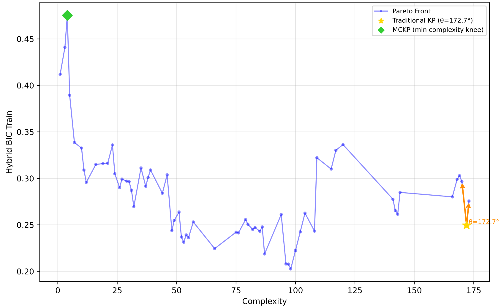
192_vineyard - Run 23 - SVP - Hybrid BIC Train \lambda_1=0.70, \bar{\lambda}_2=0.70, \lambda_3=0.90 | Difficulty: 0.67 | Method: hmr
