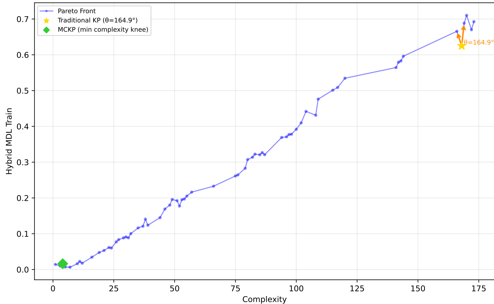
192_vineyard - Run 23 - SVP - Hybrid MDL Train \lambda_1=0.00, \bar{\lambda}_2=1.00, \lambda_3=1.00 | Difficulty: 0.67 | Method: hmr
