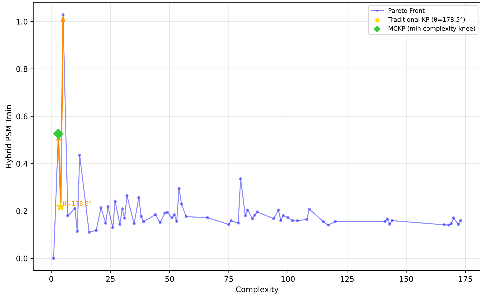
192_vineyard - Run 23 - SVP - Hybrid PSM Train \lambda_1=0.70, \bar{\lambda}_2=0.70, \lambda_3=0.90 | Difficulty: 0.67 | Method: hmr
