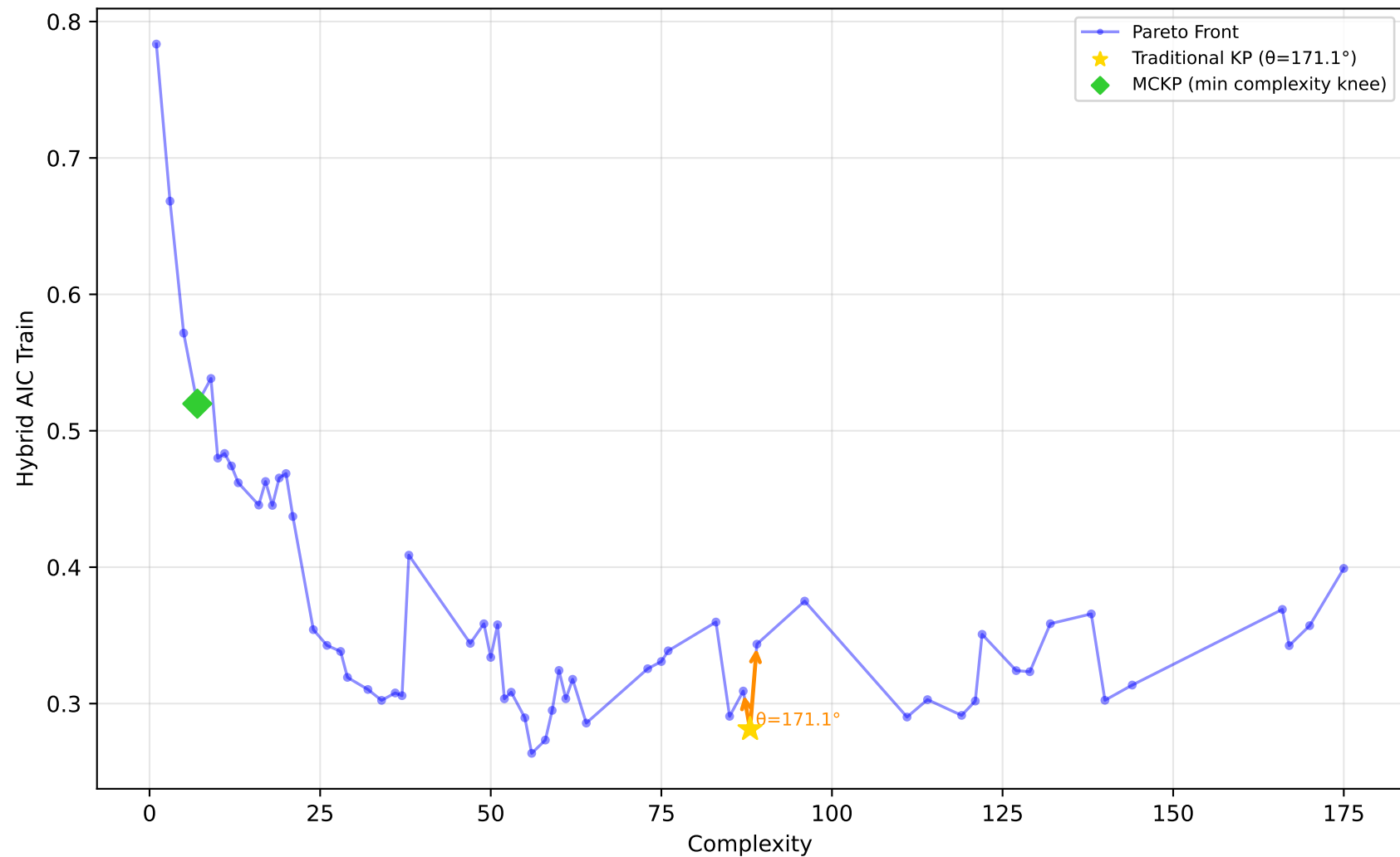
192_vineyard - Run 24 - MVP - Hybrid AIC Train \lambda_1=0.00, \lambda_2=0.30, \lambda_3=1.00 | Difficulty: 0.27 | Method: mckp
