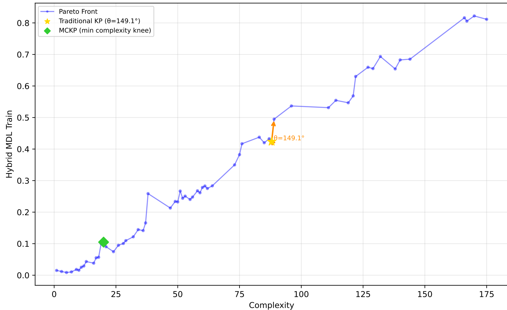
192_vineyard - Run 24 - MVP - Hybrid MDL Train \lambda_1=0.00 , \bar{\lambda}_2=0.30 , \lambda_3=1.00 | Difficulty: 0.27 | Method: mckp
