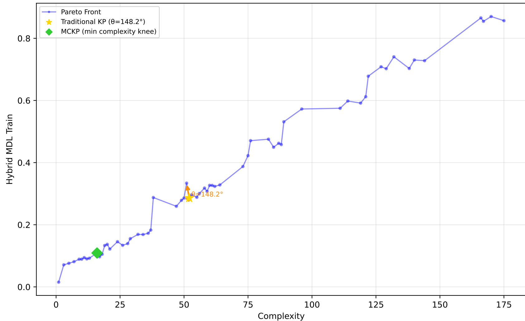
192_vineyard - Run 24 - MVP - Hybrid MDL Train \lambda_1=0.40, \bar{\lambda}_2=0.00, \lambda_3=1.00 | Difficulty: 0.27 | Method: mckp
