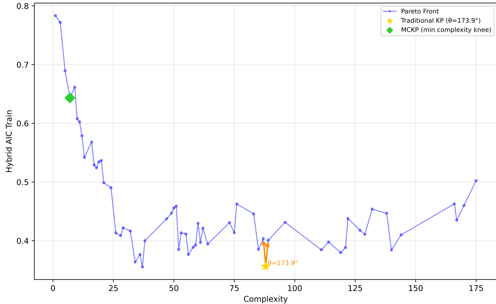
192_vineyard - Run 24 - SVP - Hybrid AIC Train \lambda_1=0.70, \lambda_2=0.70, \lambda_3=0.90 | Difficulty: 0.27 | Method: mckp
