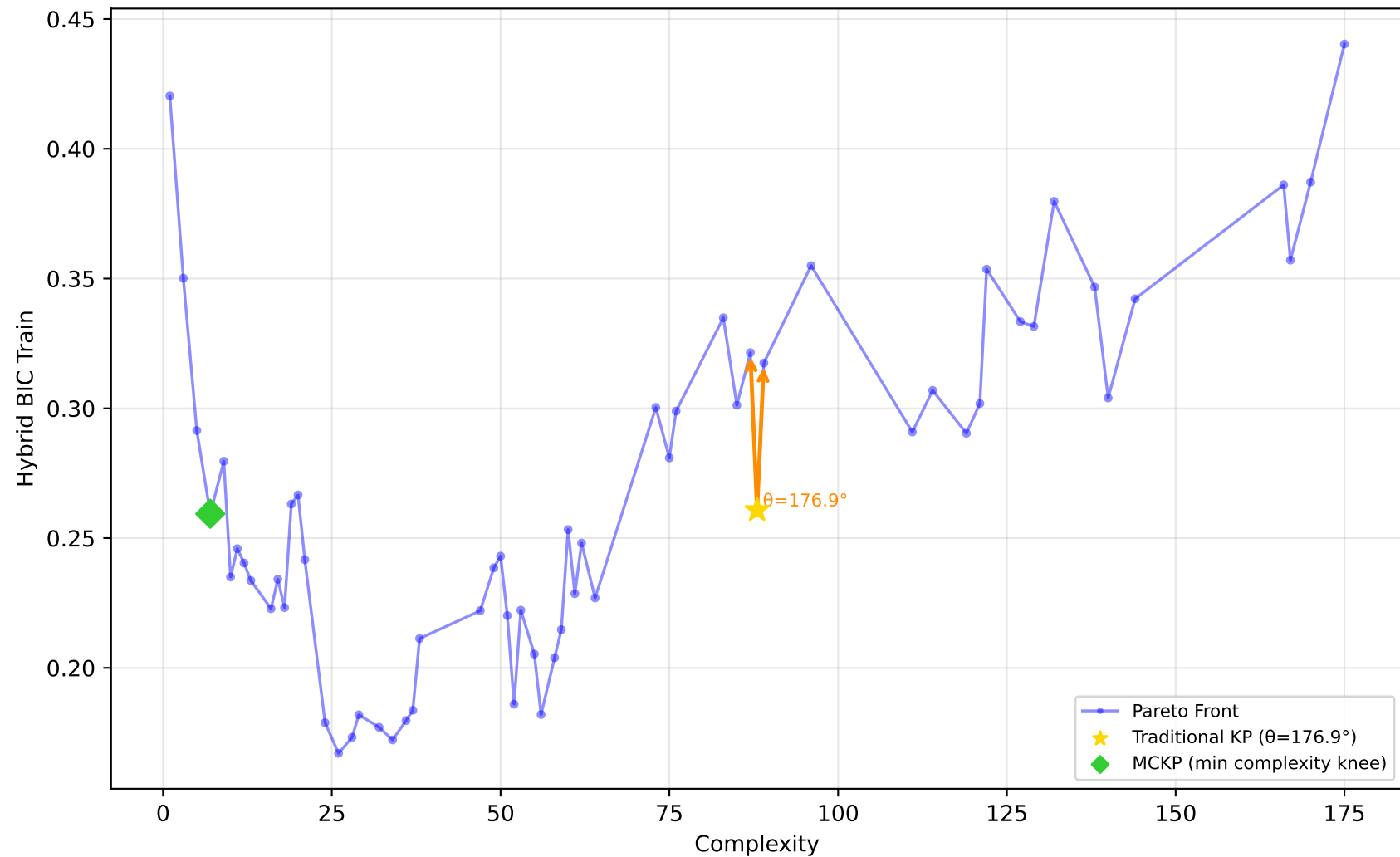
192_vineyard - Run 24 - SVP - Hybrid BIC Train \lambda_1=0.00, \lambda_2=1.00, \lambda_3=1.00 | Difficulty: 0.27 | Method: mckp
