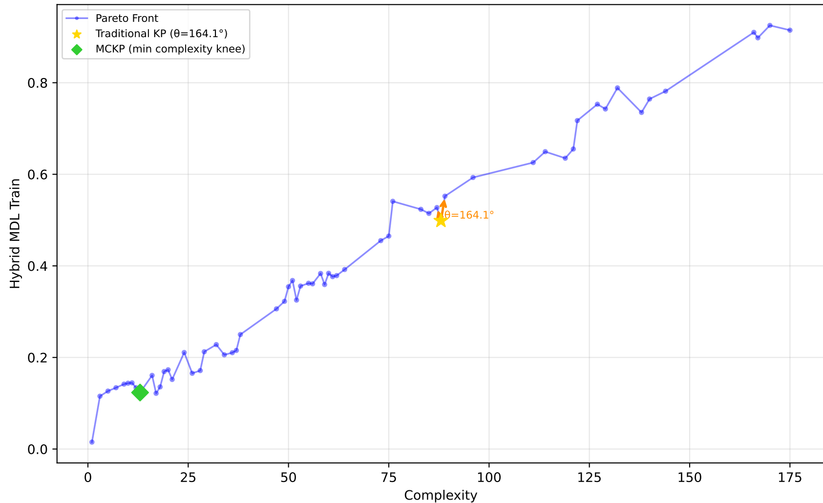
192_vineyard - Run 24 - SVP - Hybrid MDL Train \lambda_1=0.70, \lambda_2=0.70, \lambda_3=0.90 | Difficulty: 0.27 | Method: mckp
