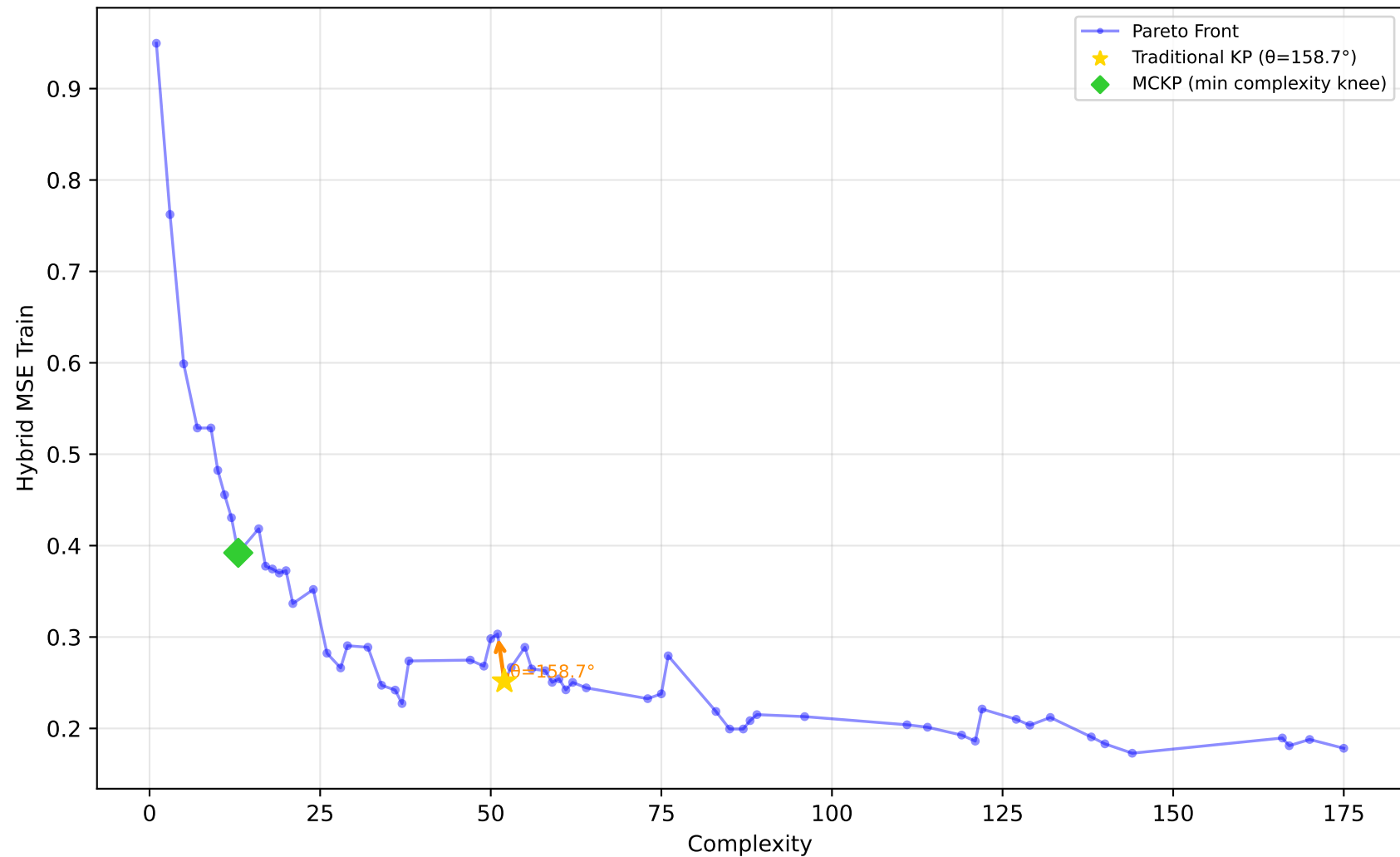
192_vineyard - Run 24 - SVP - Hybrid MSE Train \lambda_1=0.70, \lambda_2=0.70, \lambda_3=0.90 | Difficulty: 0.27 | Method: mckp
