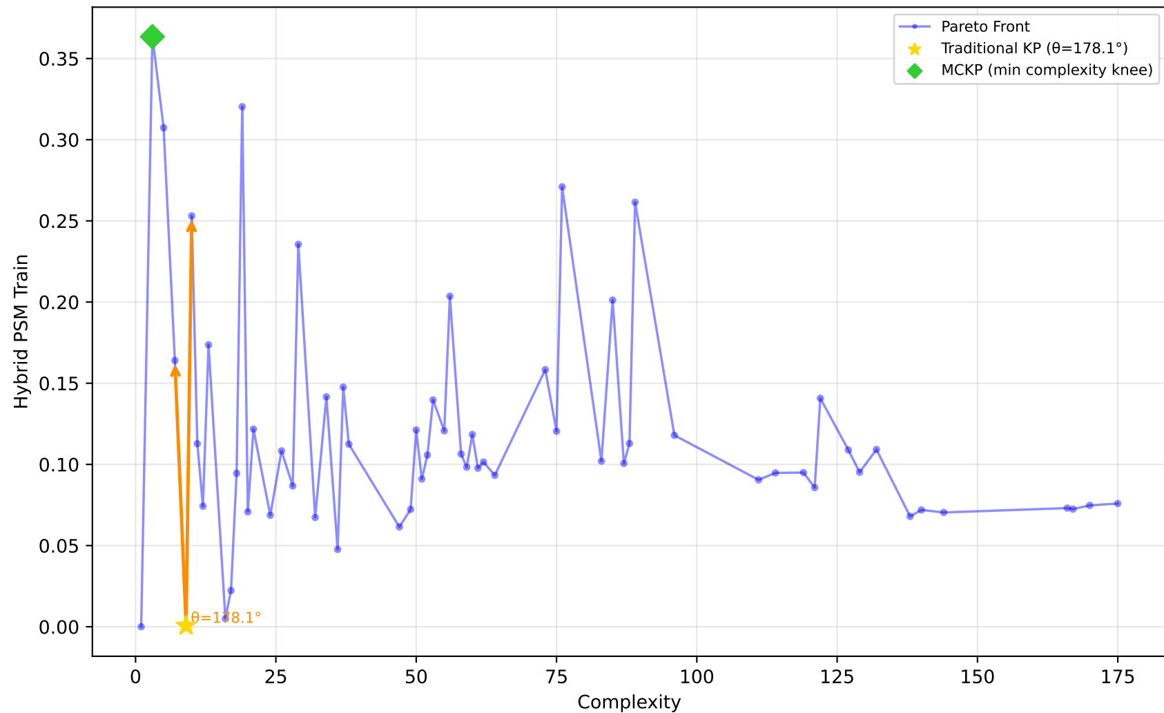
192_vineyard - Run 24 - SVP - Hybrid PSM Train \lambda_1=0.00, \lambda_2=1.00, \lambda_3=1.00 | Difficulty: 0.27 | Method: mckp
