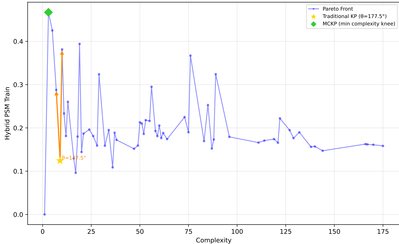
192_vineyard - Run 24 - SVP - Hybrid PSM Train \lambda_1=0.70, \lambda_2=0.70, \lambda_3=0.90 | Difficulty: 0.27 | Method: mckp
