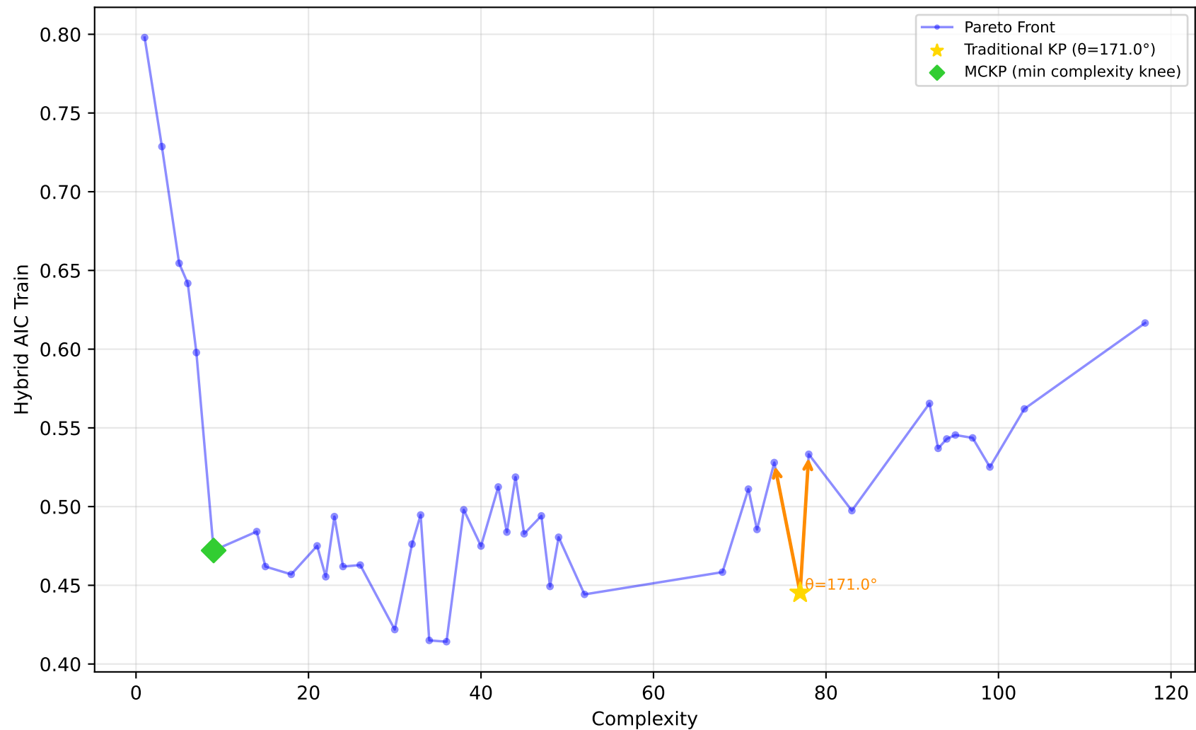
192_vineyard - Run 25 - MVP - Hybrid AIC Train \lambda_1=0.40 , \bar{\lambda}_2=0.00 , \lambda_3=1.00 | Difficulty: 1.00 | Method: hmr
