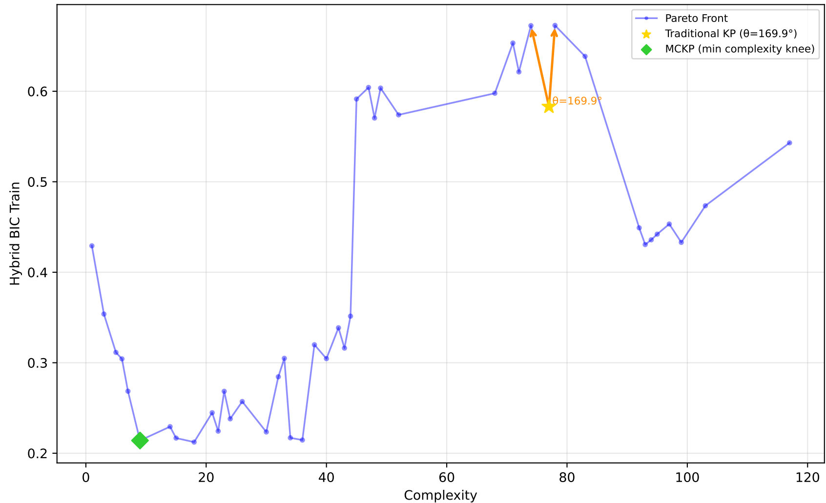
192_vineyard - Run 25 - MVP - Hybrid BIC Train \lambda_1=0.00, \bar{\lambda}_2=0.30, \lambda_3=1.00 | Difficulty: 1.00 | Method: hmr
