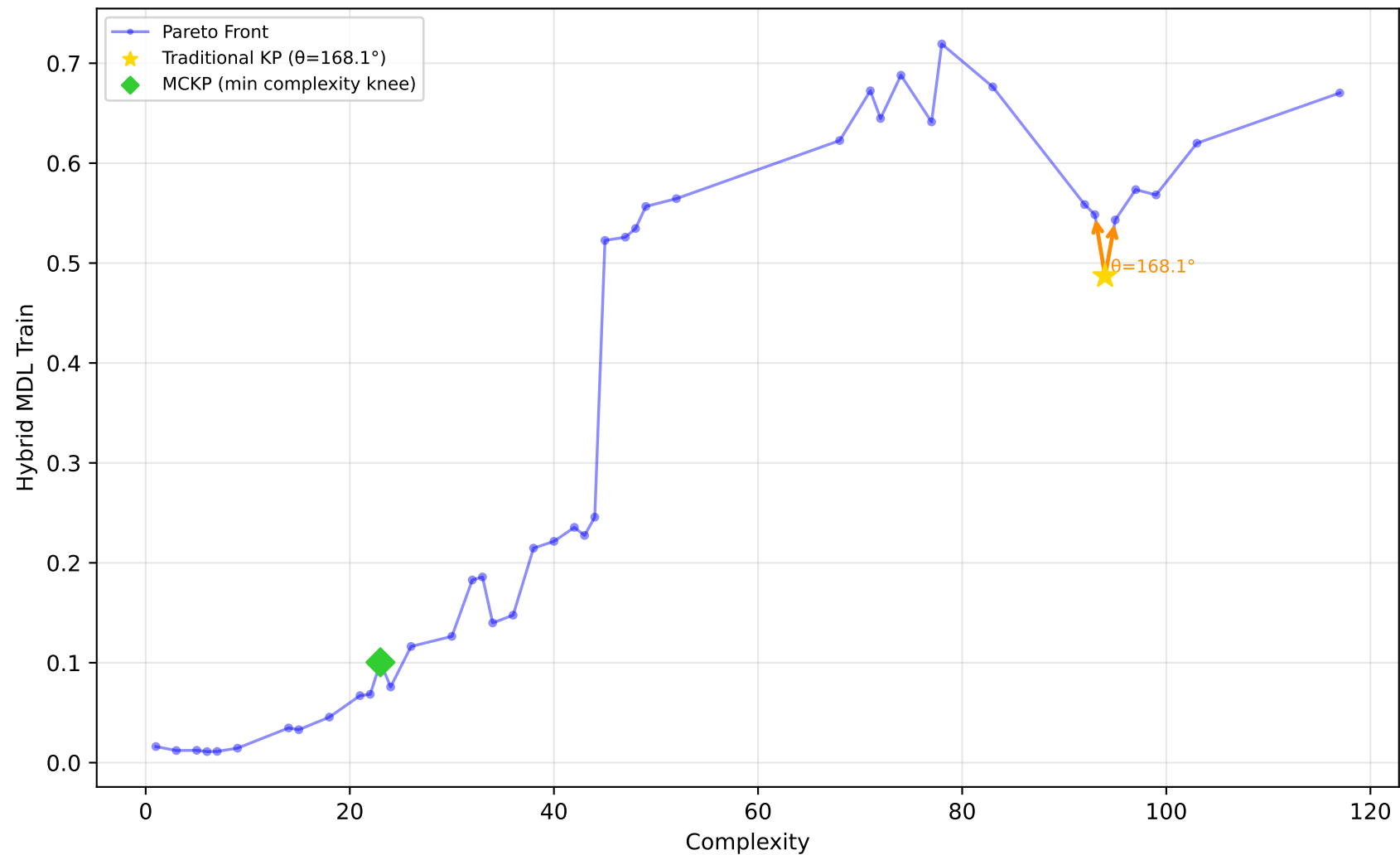
192_vineyard - Run 25 - MVP - Hybrid MDL Train \lambda_1=0.00, \lambda_2=0.30, \lambda_3=1.00 | Difficulty: 1.00 | Method: hmr
