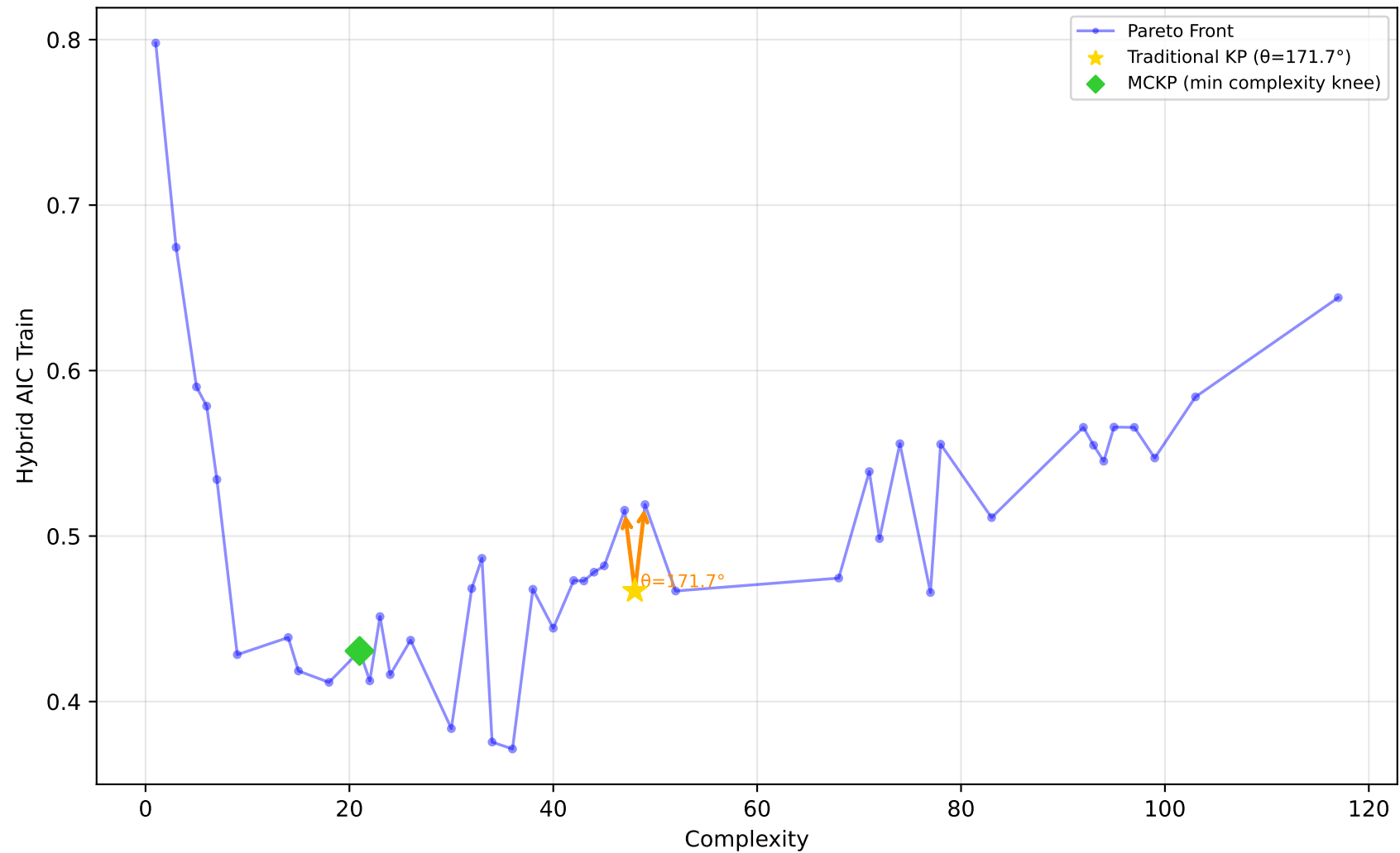
192_vineyard - Run 25 - SVP - Hybrid AIC Train \lambda_1=0.00, \lambda_2=1.00, \lambda_3=1.00 | Difficulty: 1.00 | Method: hmr
