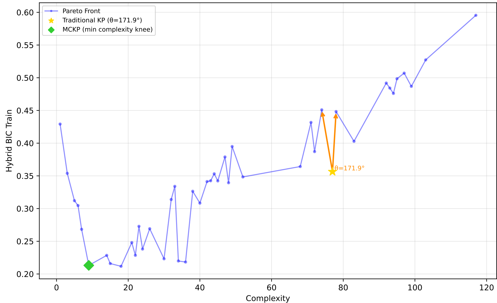
192_vineyard - Run 25 - SVP - Hybrid BIC Train \lambda_1=0.00, \bar{\lambda}_2=1.00, \lambda_3=1.00 | Difficulty: 1.00 | Method: hmr
