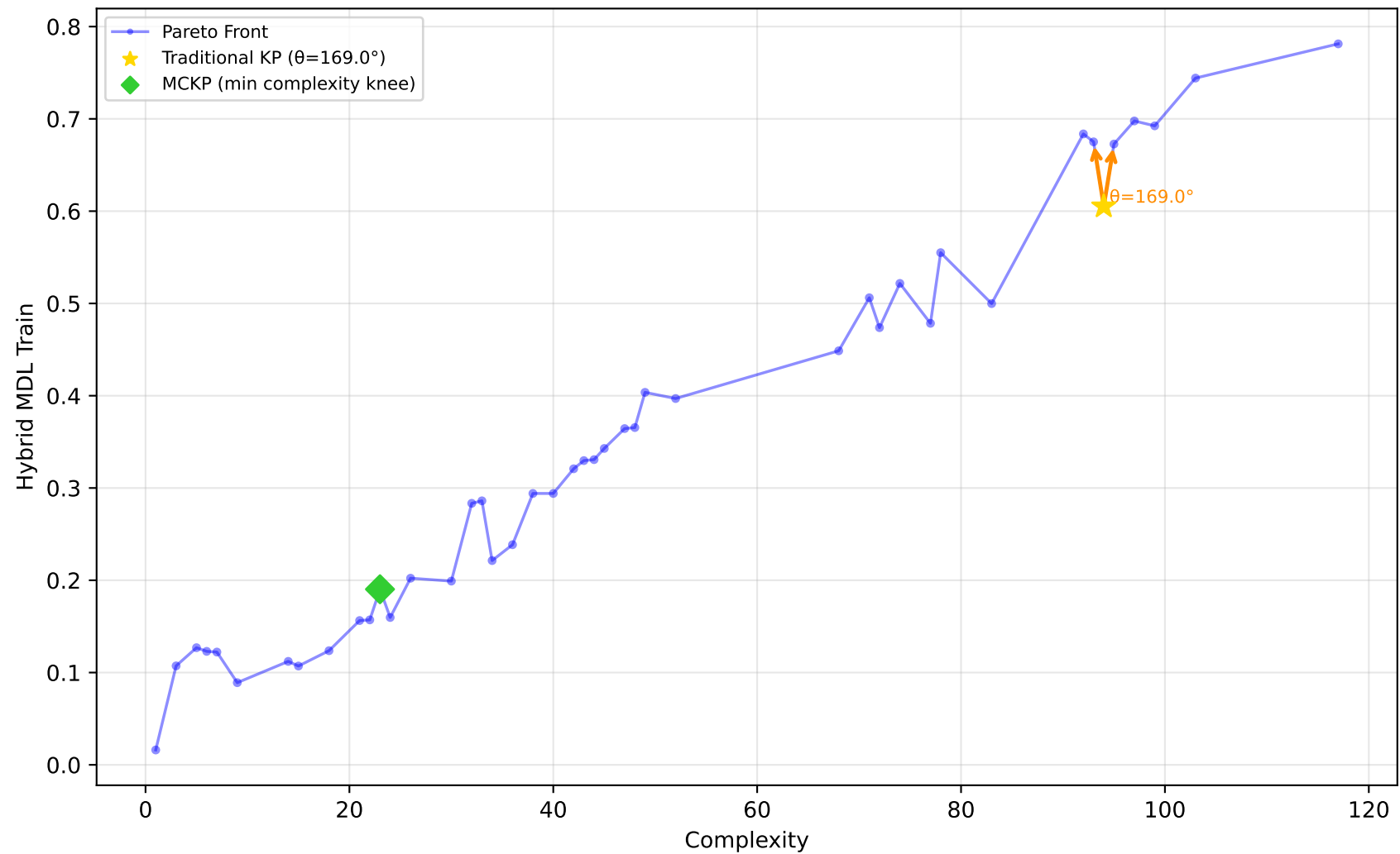
192_vineyard - Run 25 - SVP - Hybrid MDL Train \lambda_1=0.70, \bar{\lambda}_2=0.70, \lambda_3=0.90 | Difficulty: 1.00 | Method: hmr
