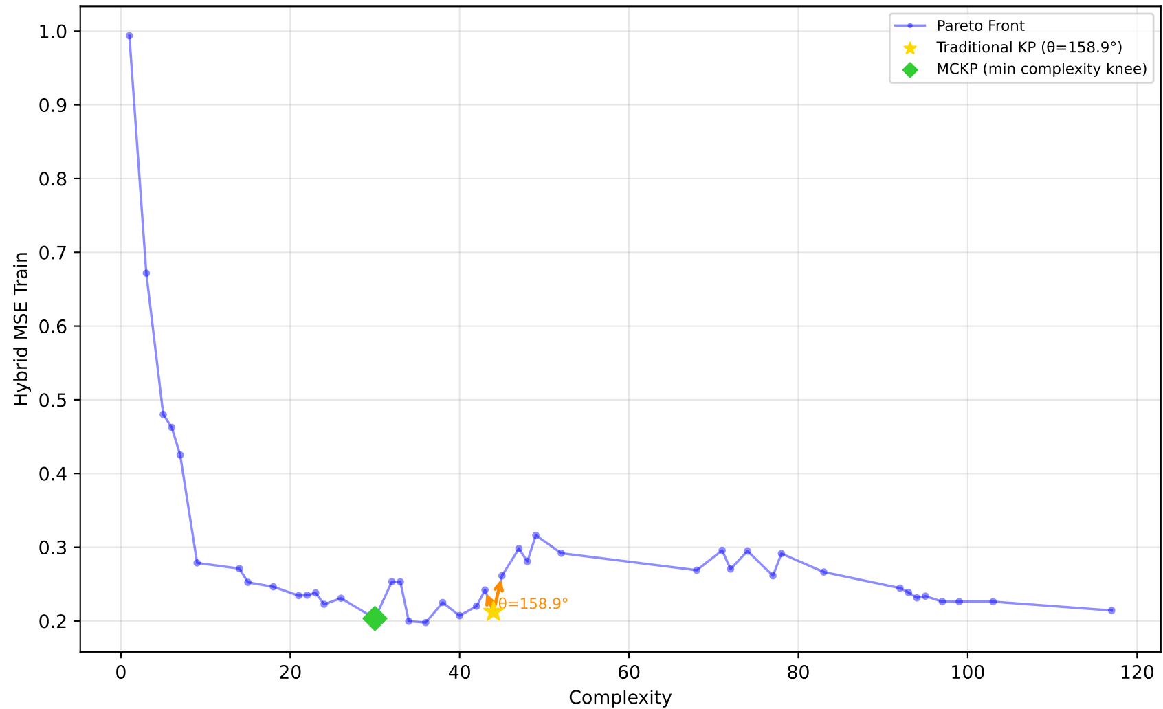
192_vineyard - Run 25 - SVP - Hybrid MSE Train \lambda_1=0.00, \lambda_2=1.00, \lambda_3=1.00 | Difficulty: 1.00 | Method: hmr
