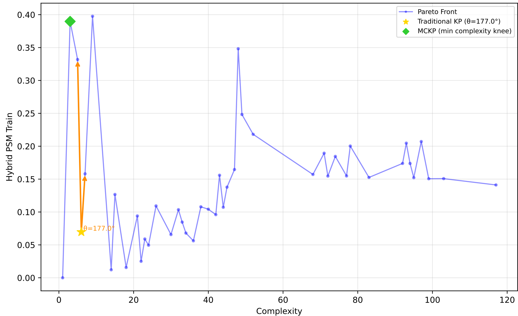
192_vineyard - Run 25 - SVP - Hybrid PSM Train \lambda_1=0.00 , \bar{\lambda}_2=1.00 , \lambda_3=1.00 | Difficulty: 1.00 | Method: hmr
