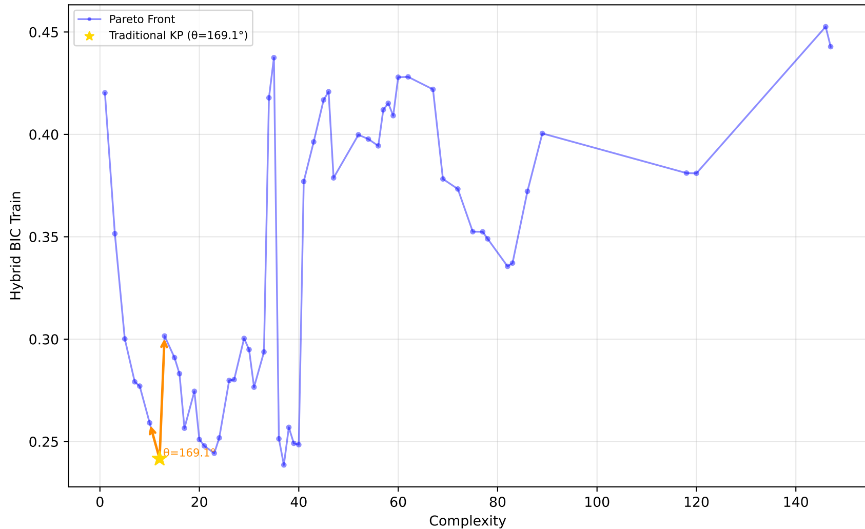
192_vineyard - Run 26 - MVP - Hybrid BIC Train \lambda_1=0.00, \lambda_2=0.30, \lambda_3=1.00 | Difficulty: 0.32 | Method: mckp
