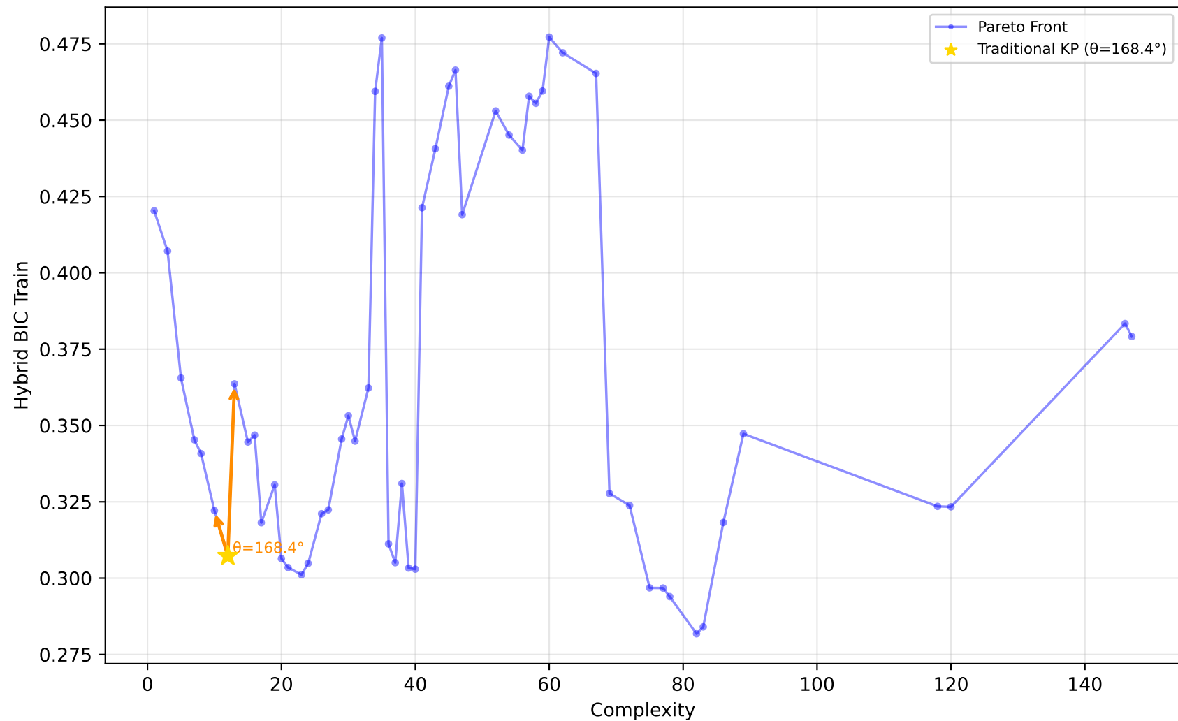
192_vineyard - Run 26 - MVP - Hybrid BIC Train \lambda_1=0.40 , \lambda_2=0.00 , \lambda_3=1.00 | Difficulty: 0.32 | Method: mckp
