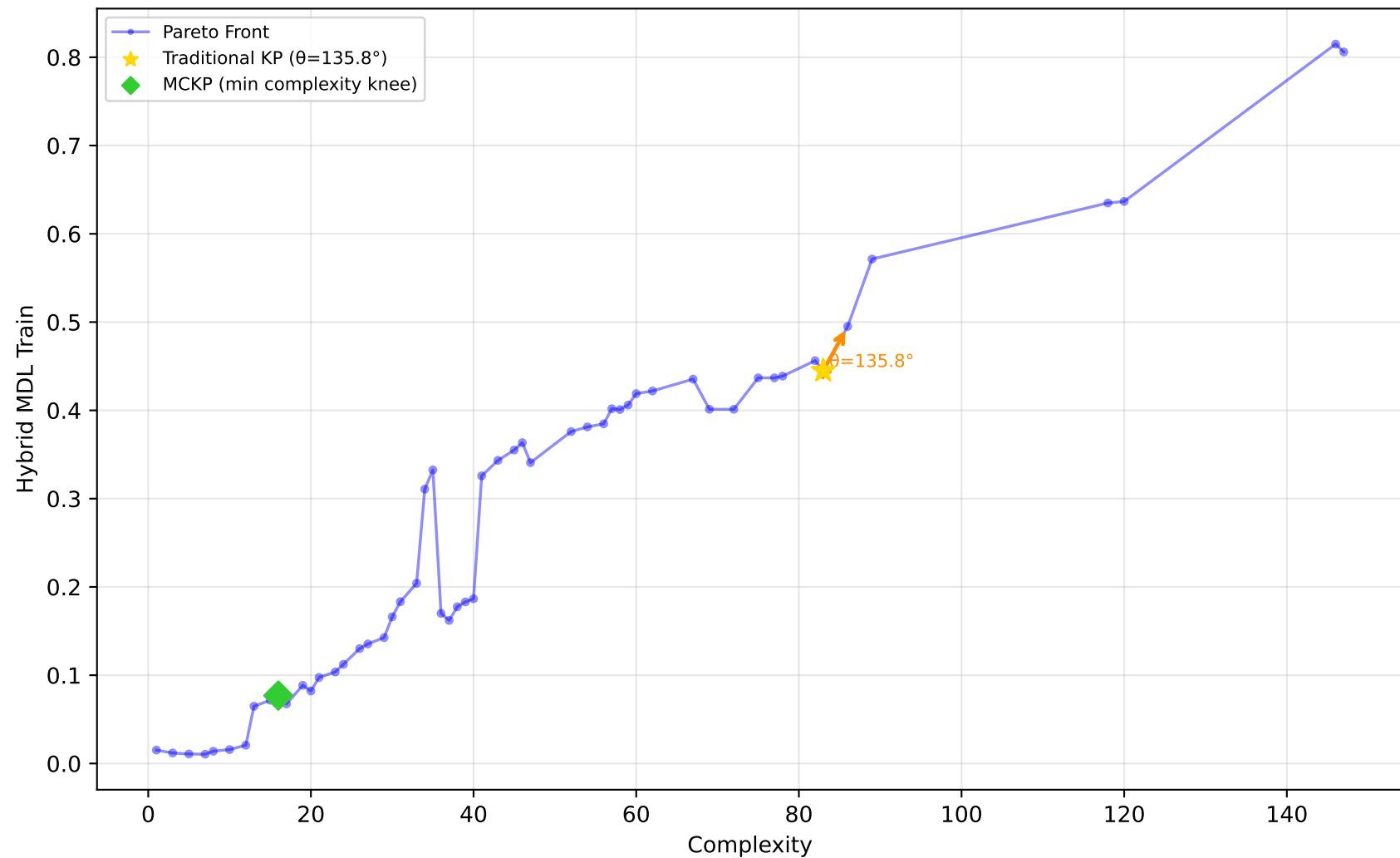
192_vineyard - Run 26 - MVP - Hybrid MDL Train \lambda_1=0.00, \bar{\lambda}_2=0.30, \lambda_3=1.00 | Difficulty: 0.32 | Method: mckp
